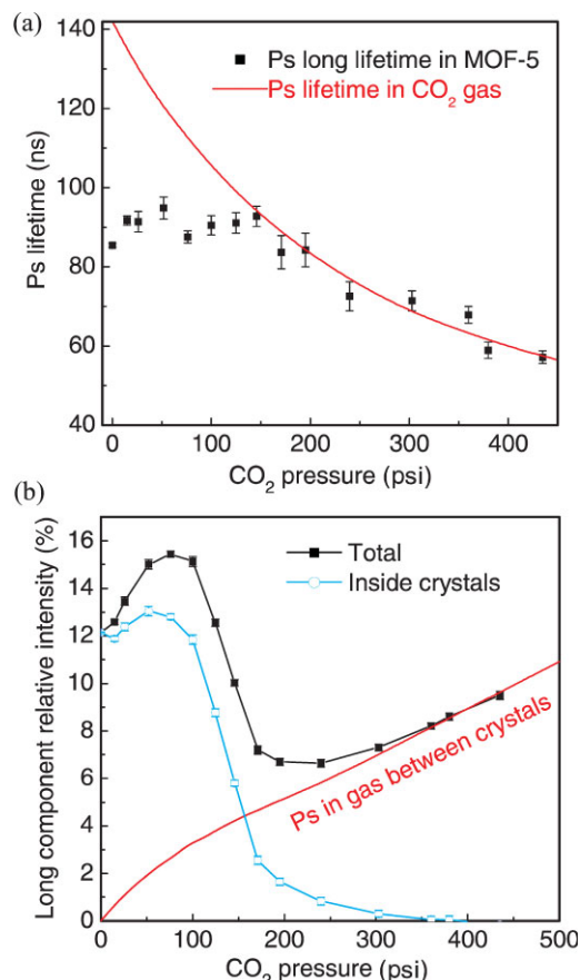
Figure 3. The evolution of the long-lived (defect) Ps component of MOF-5 versus CO 2 pressure. a) The Ps lifetimes and b) the corresponding relative intensities. This Ps component evidently has two origins in MOF-5: Ps annihilating in 6-nm defects with intensities plotted in (b) with open symbols (the result of subtracting the smooth curve from the total intensities) and Ps formed and annihilating in the CO 2 gas surrounding the crystal grains.
